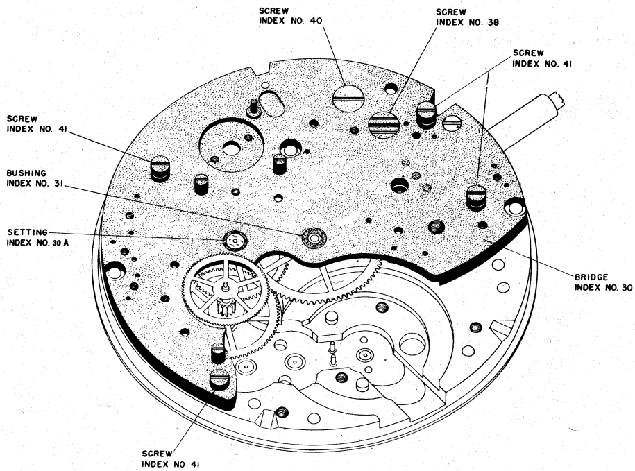
Figure 6. Barrel bridge assembly.
